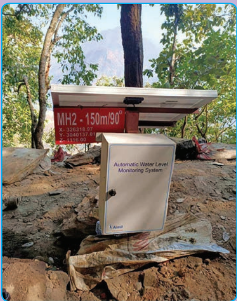
Installation of Automatic Data Logger for Vibrating Wire Piezometer (KTFT Project)
